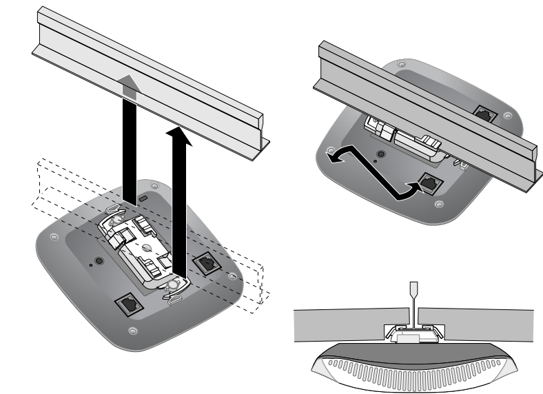
Figure 8 Mounting the IAP
