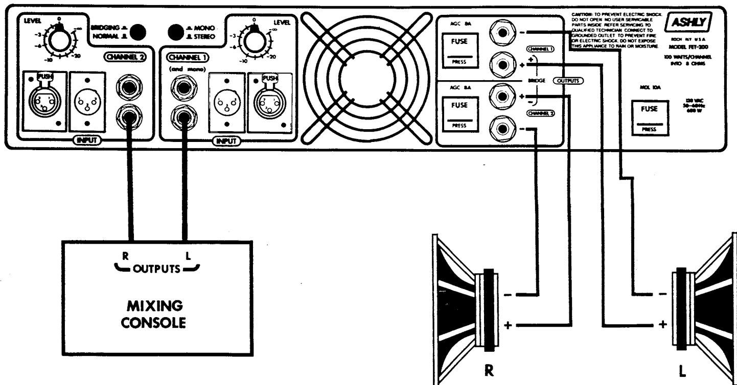
Figure 4 Stereo Operation
