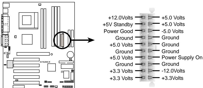
A7A266-E ATX Power Connector
