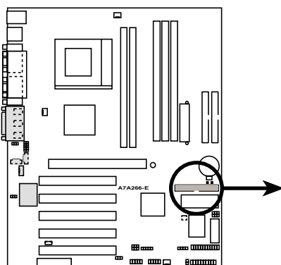
A7A266-E Floppy Disk Drive Connector
