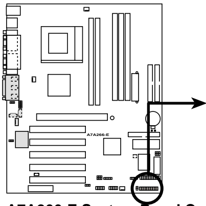
A7A266-E System Panel Connectors
