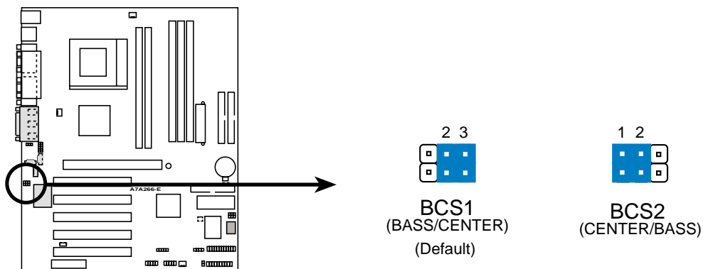
A7A266-E Jumper Mode Setting
