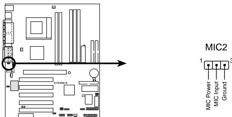
A7A266-E Internal Microphone Connector
