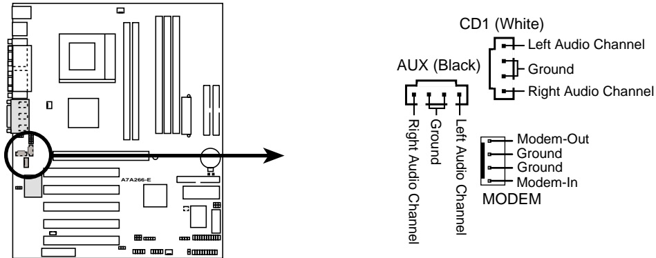
A7A266-E Internal Audio Connectors
