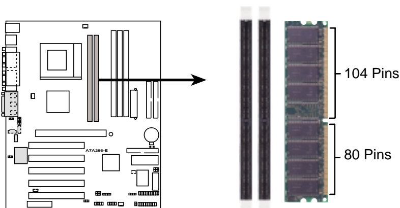
A7A266-E 184-Pin DDR DIMM Sockets
