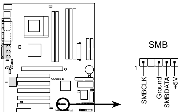
A7A266-E SMBus Connector
