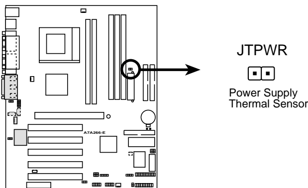
A7A266-E Thermal Sensor Connector
