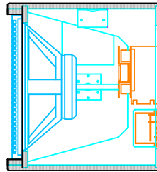
SECTION VIEW
