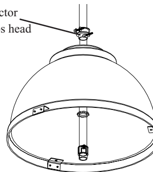
Figure 1 Slide housing and connector onto conduit
