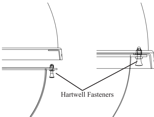
Figure 5 Attach the dome to the housing
