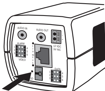
Figure 5.10 Reset button
