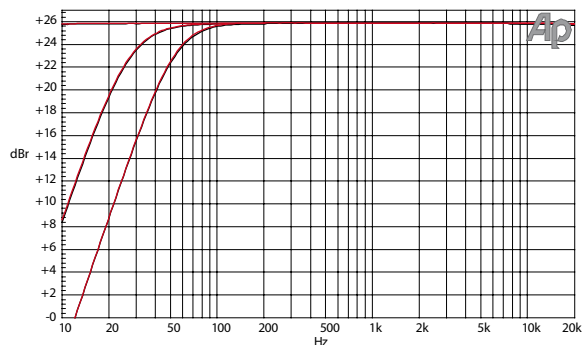
Figure 8.2 Gain vs. frequency / Different positions of HPF-Switch (Ch1, Ch2) (Measurements of a typical performance)
