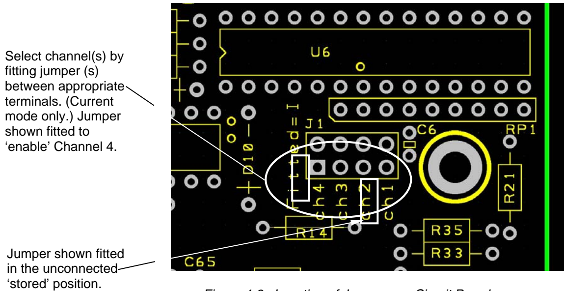
Figure 4-3. Location of Jumpers on Circuit Board
