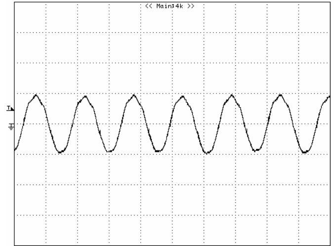
Figure 11: Input Terminal Ripple Current, i_c , at full rated output current and nominal input voltage with 12 \mu H source impedance and 33 \mu F electrolytic capacitor (500 mA/div).
