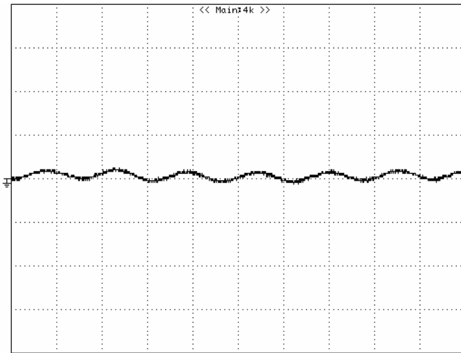
Figure 12: Input reflected ripple current, i_s , through a 12 \mu H source inductor at nominal input voltage and rated load current (20 mA/div).
