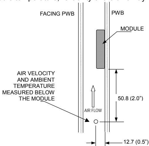
Figure 19: Wind Tunnel Test Setup
