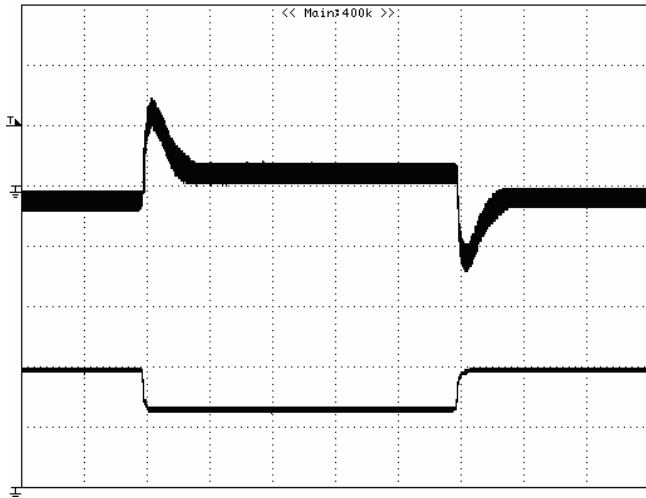
Figure 8: Output voltage response to step-change in load current Iout1 (75%-50%-75% of Io, max; di/dt = 0.1A/μs, 200uS/DIV). Vin=48V. Load cap: 10μF, tantalum capacitor and 1μF ceramic capacitor. Top trace: Vout (100mV/div), Bottom trace: Iout (1A/div). Scope measurement should be made using a BNC cable (length short than 20 inch). Position the load between 51 mm and 76 mm (2inch and 3 inch) from the module.
