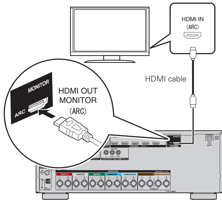
Receiver (Rear panel)
